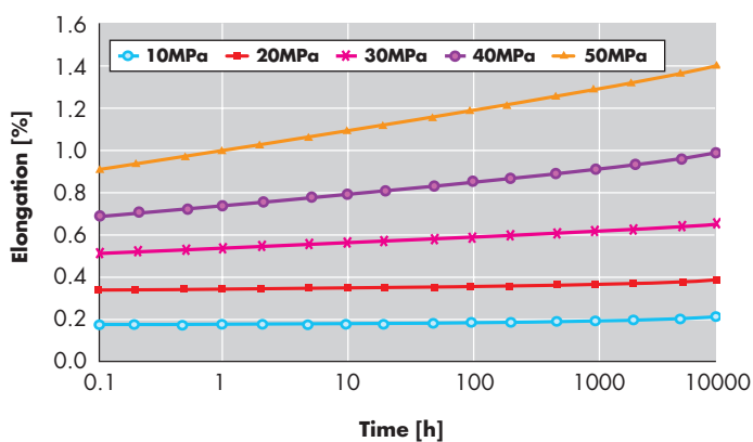
Creep curves Grilon TSG-30/4 at 23°C / 50% r.h.
