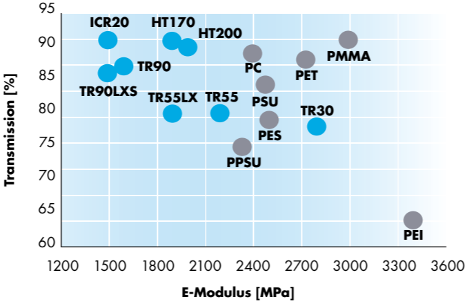
Transmission measured on 3 mm thick plates at 560 nm
