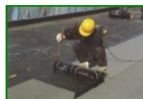
Modified-asphalt sheeting
