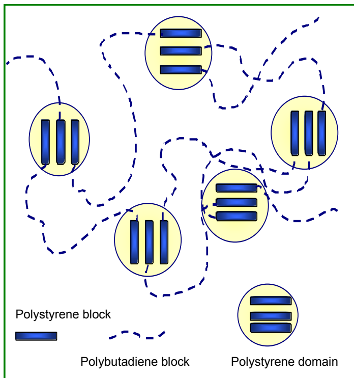
Typical SBS structure
