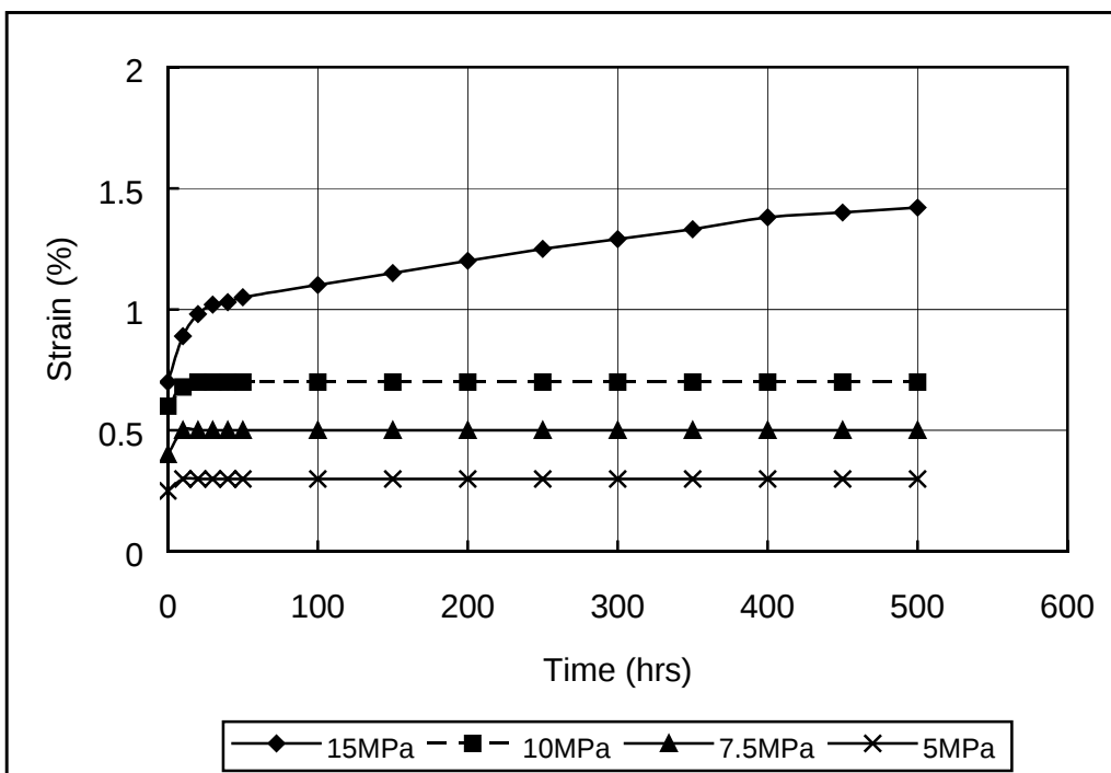
Fig 1-4 Creep Property of “TOYOLAC” 100
