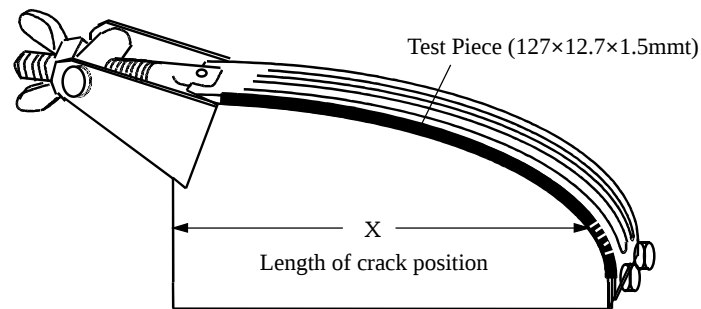
Figure of 1/4 Ellipse-Jig
