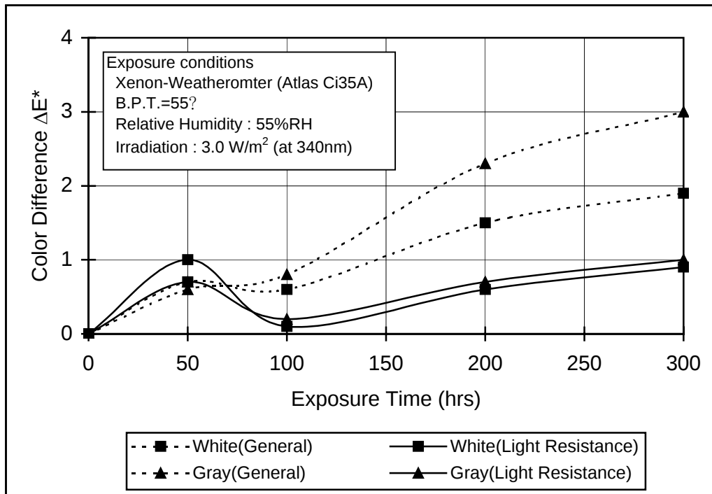
Fig 1-5 Light resistance performance of "TOYOLAC" 700 -314
