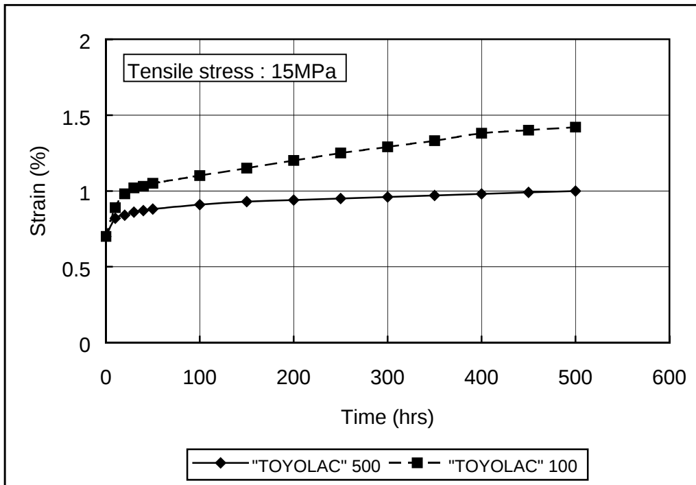
Fig 1-3 Creep Property of “TOYOLAC” 100 & 500
