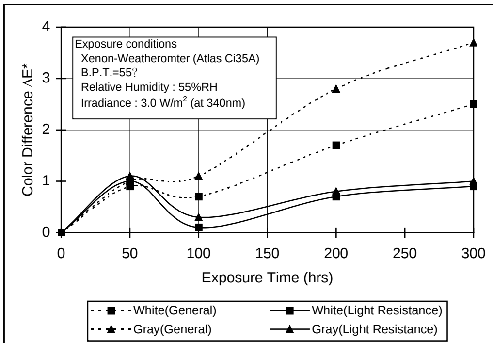
Fig 1-6 Light resistance performance of "TOYOLAC" 100 -322
